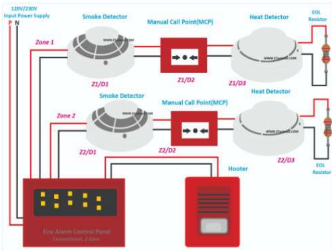
Conventional Fire Alarm System
