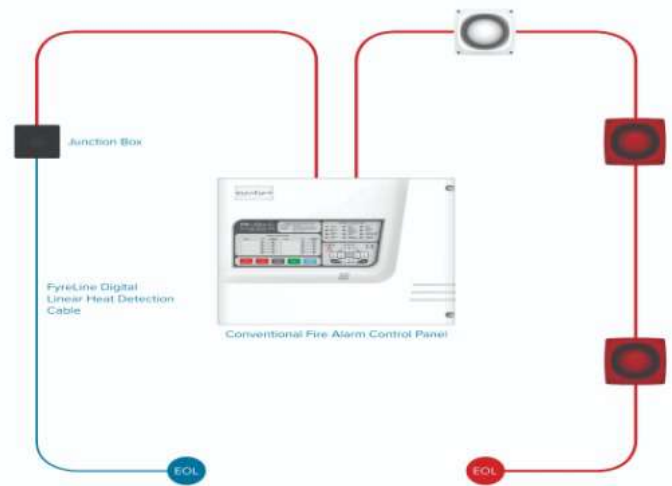
Digital Linear Heat Detection System
