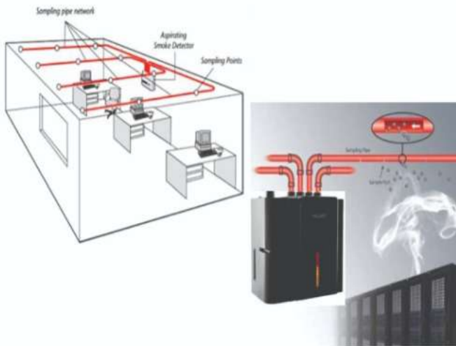
Aspiration System
