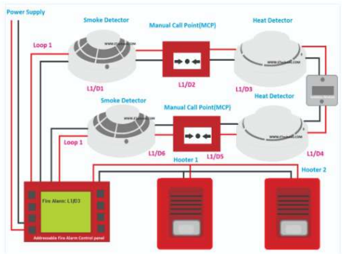
Addressable Fire Alarm System
